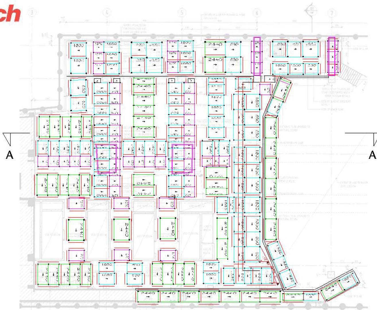
BASEMENT 1 SLAB
